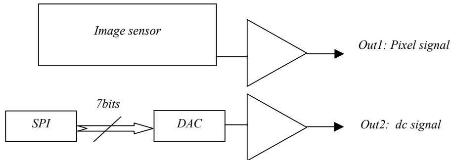
Figure 5: Output stage architecture
