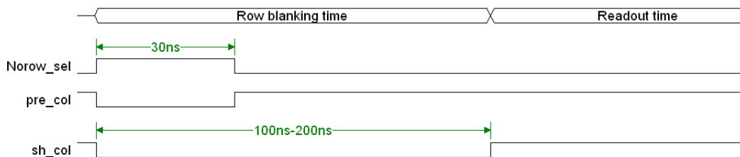
Figure 19: Reduced standard ROT by means of Sh_col signal. pre_col (short pulse) , Norowsel (short pulse) and Sh_col (large pulse).
