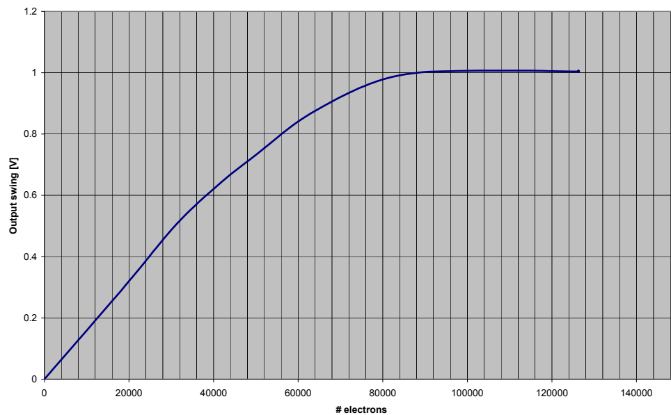
Figure 2: Photo-voltaic response curve
