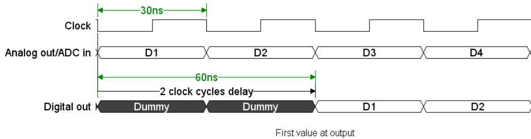
Figure 6: ADC timing
