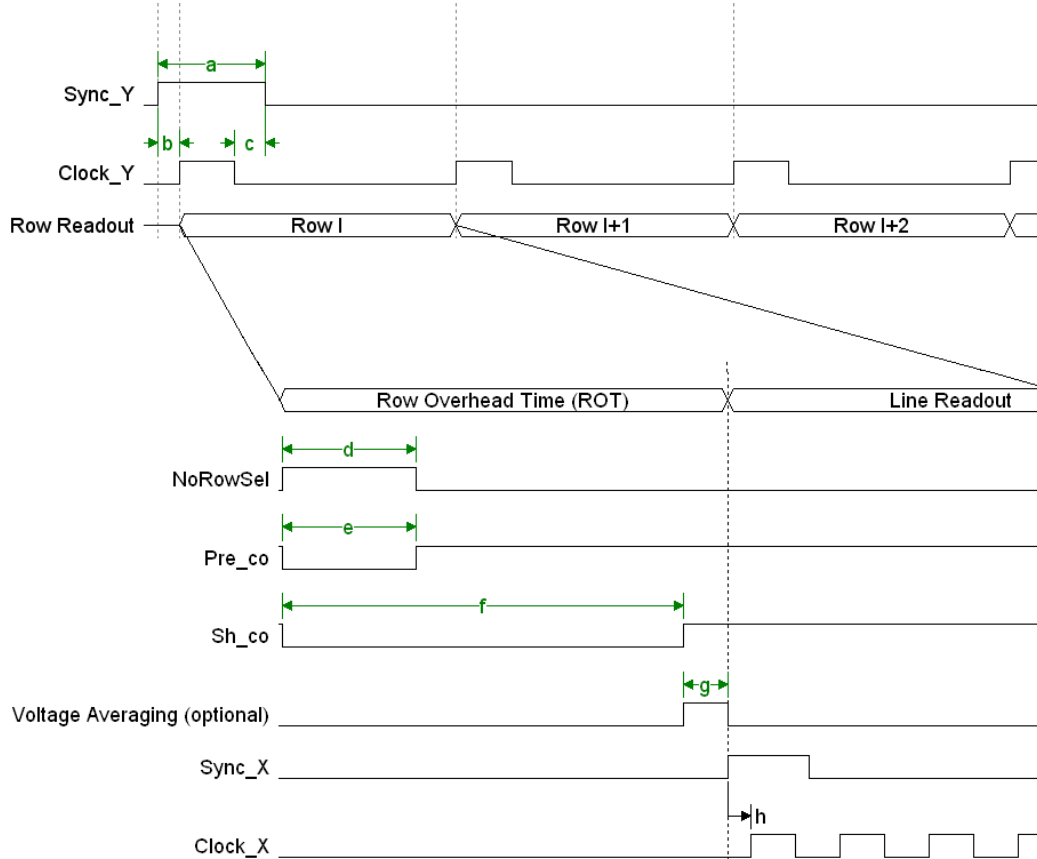
Figure 15: X- and Y-addressing
