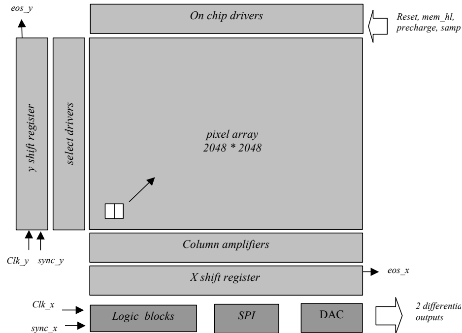
Figure 3: Block diagram of the image sensor
