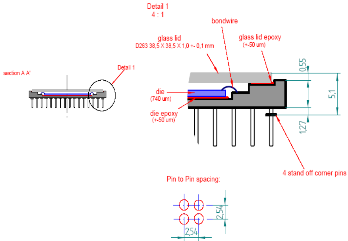
Figure 23: LUPA-4000 package specifications with die
