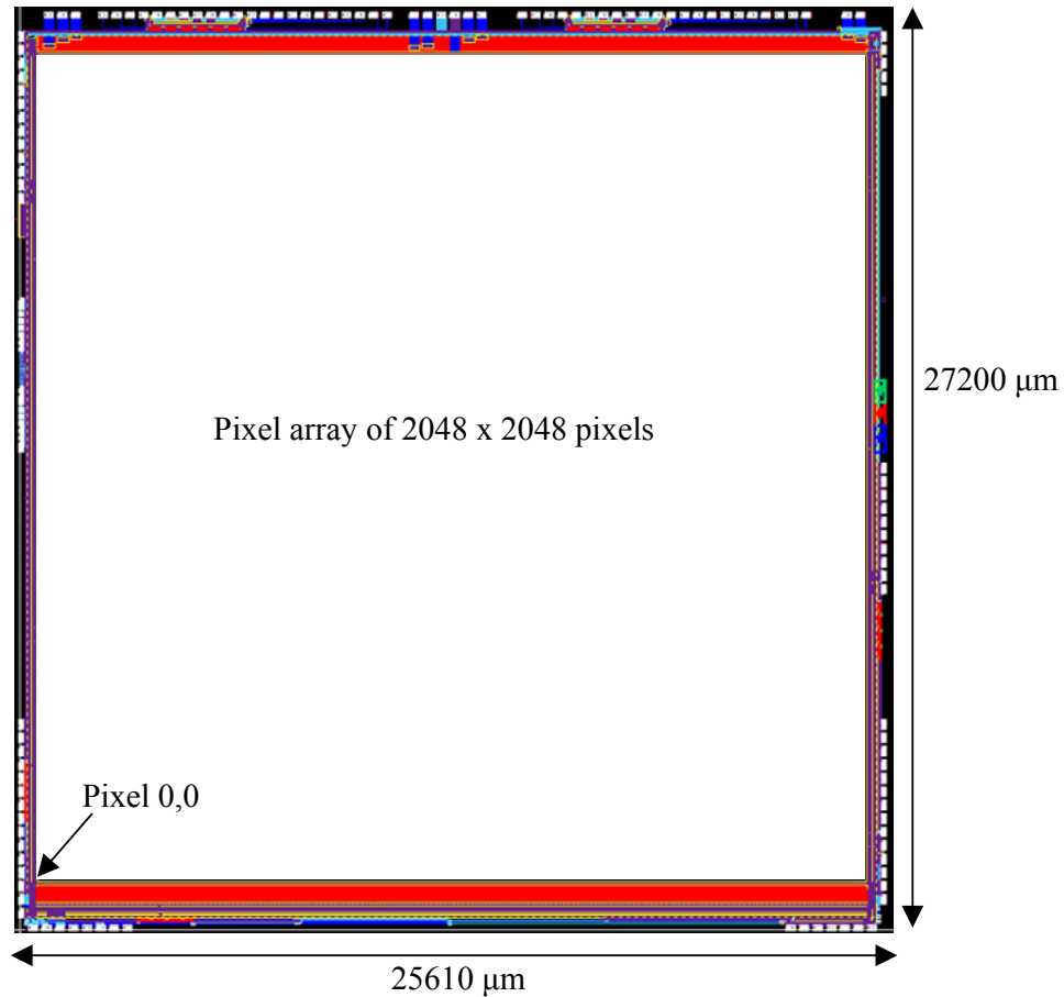
Figure 21: Die figure of the LUPA-4000
