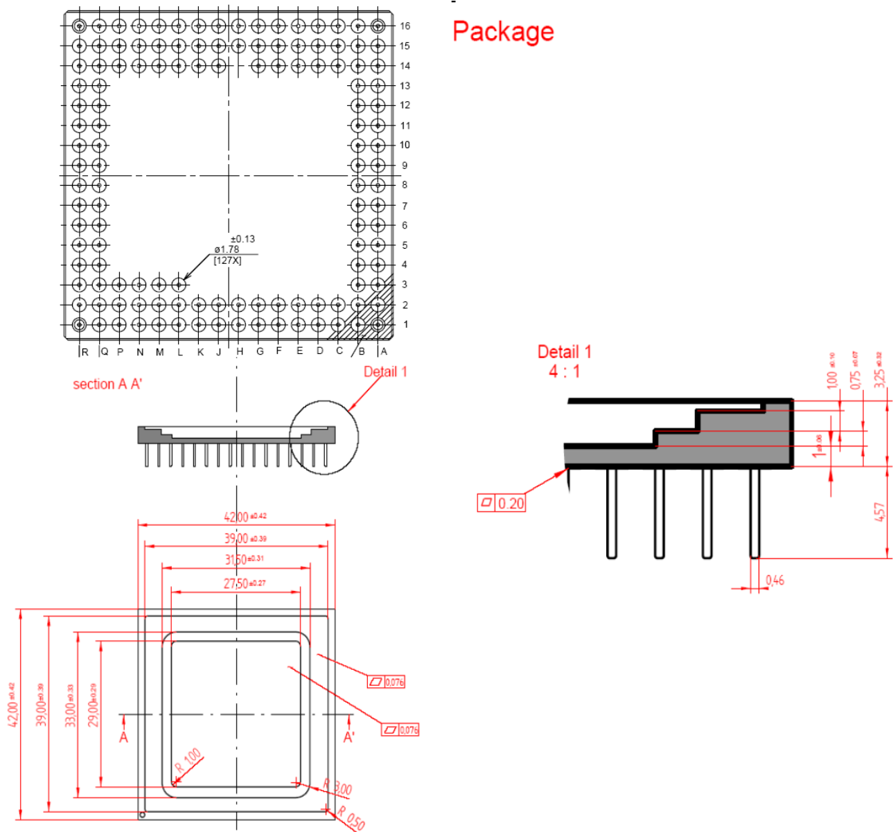
Figure 22: Package drawing of the LUPA-4000 package
