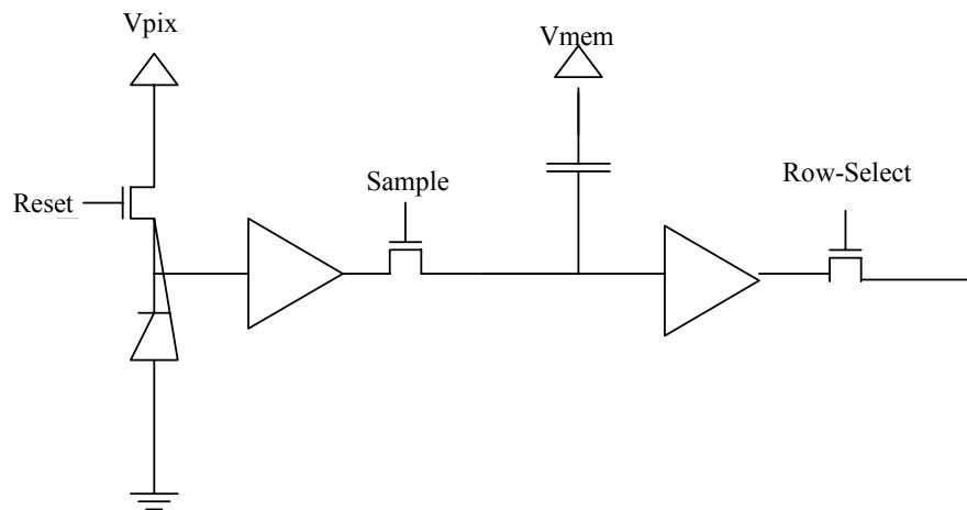
Figure 4: 6T-pixel architecture
