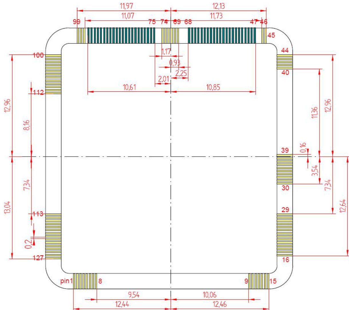
Figure 24: Placing of the bonding pads on the LUPA-4000 package
