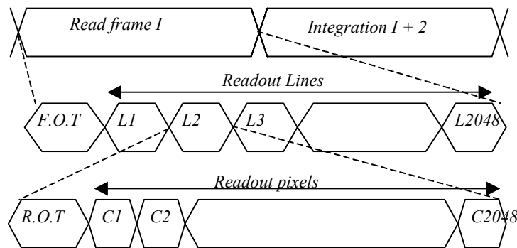
Figure 14: Readout of the image sensor. F.O.T: Frame overhead time. R.O.T: Row overhead time. L: selection of line, C: Selection of column.
