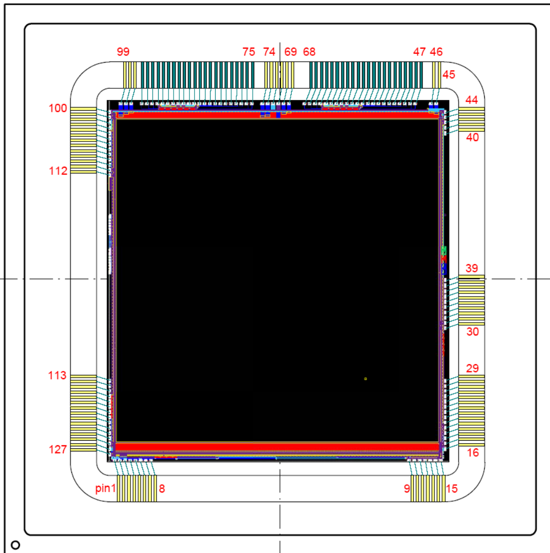
Figure 25: Bonding pads diagram of the LUPA-4000 package
