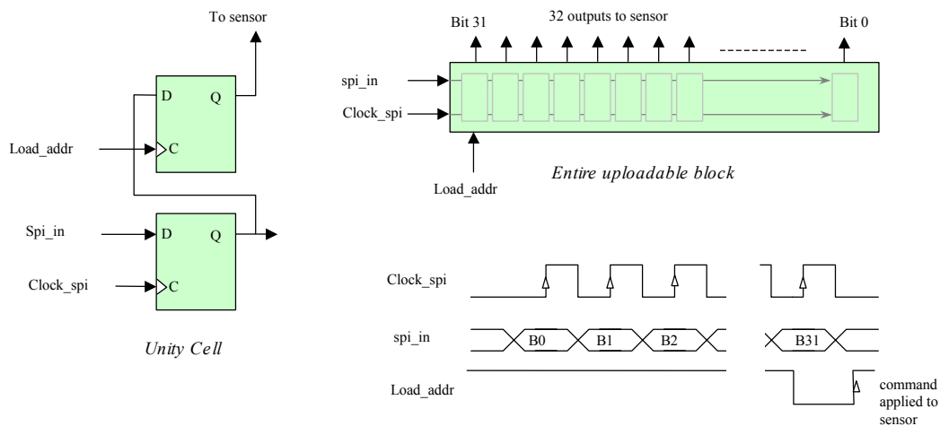
Figure 20: SPI block diagram and timing
