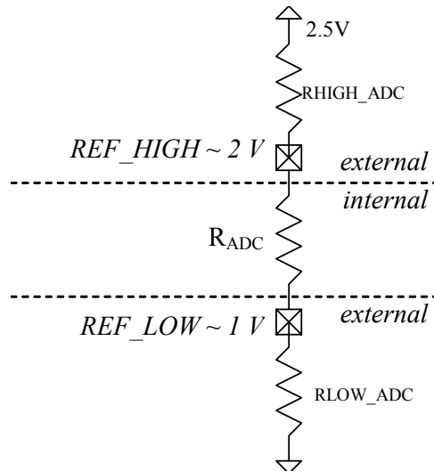
Figure 7: In- and external ADC connections
