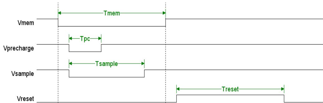
Figure 10: Internal timing of the pixel. Levels are defined by the pixel array voltage supplies (For the correct polarities of the signals refer to table 11).
