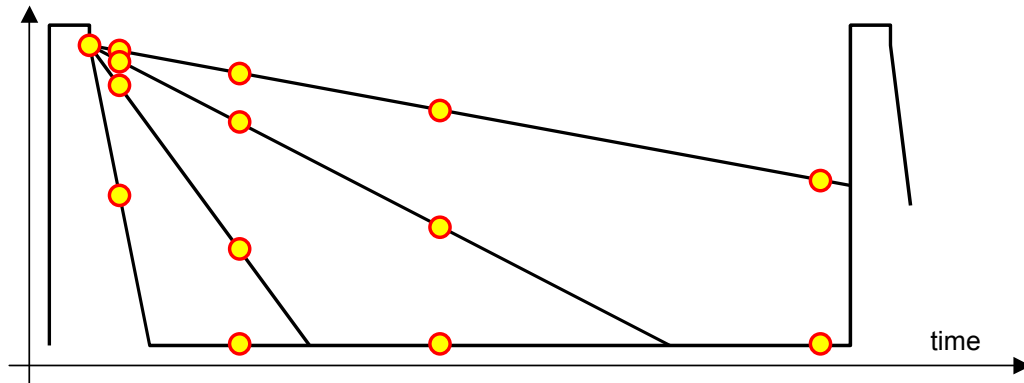
Figure 9. Principle of non-destructive readout.
