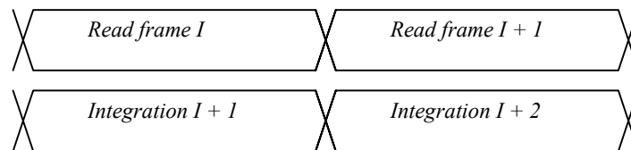
Figure 11: Integration and read out in parallel
