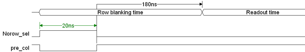
Figure 18: Standard timing for the R.O.T. Only pre_col and Norowsel control signals are required.
