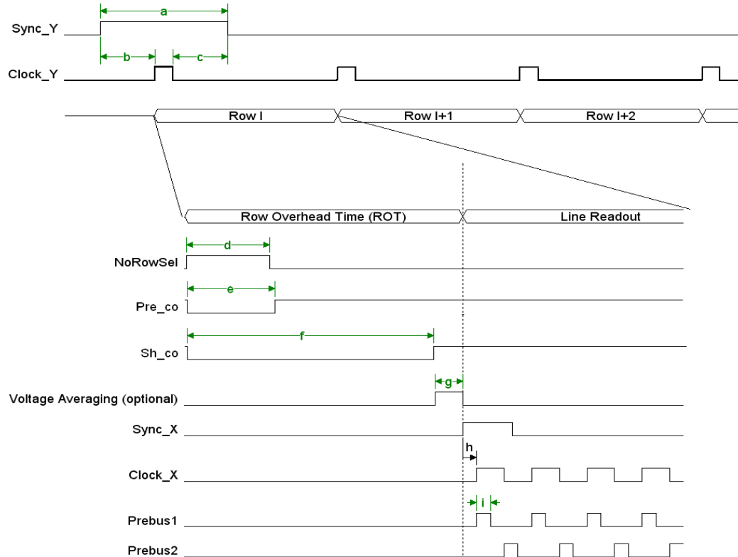
Figure 20: X- and Y-addressing with precharging of the buses
