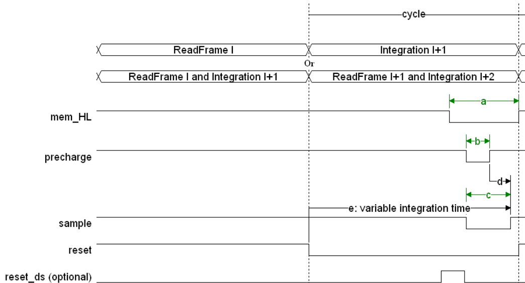
Figure 13: Timing of the pixel array: The integration time is determined by the falling edge of the reset pulse. The longer the pulse is high, the shorter the integration time. At the end of the integration time, the information has to be stored onto the memory element for readout.
