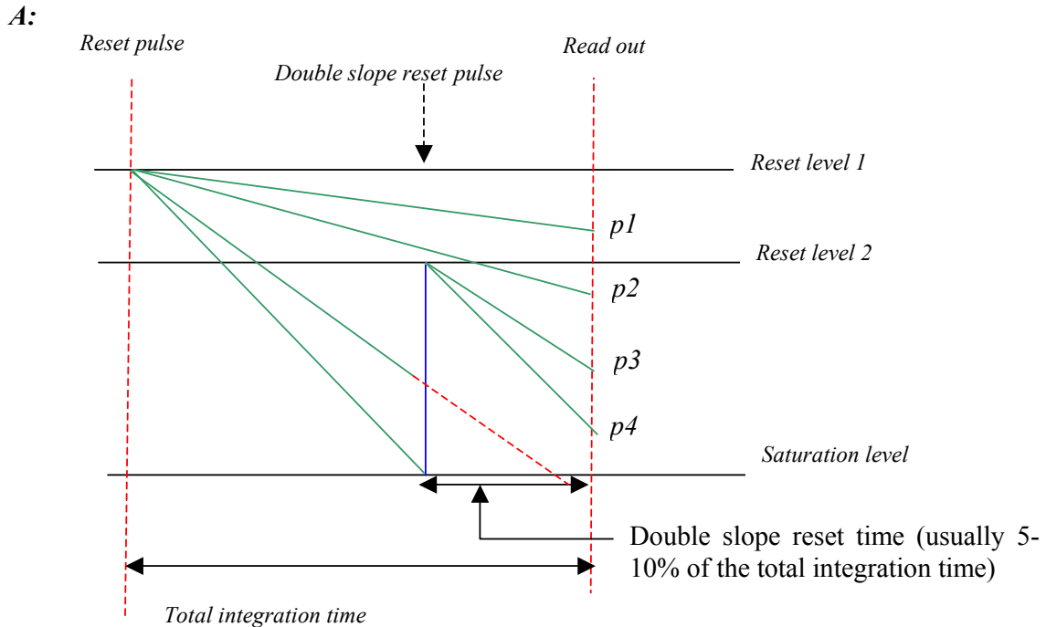
Figure 21: Dual slope diagram
