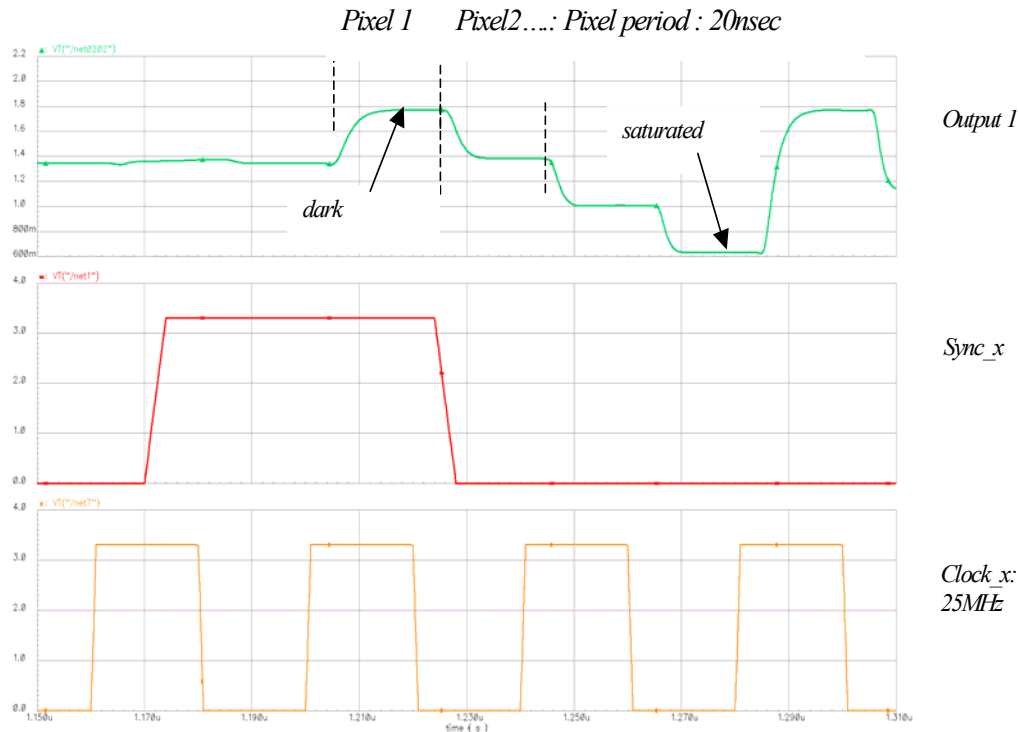
Figure 17: output signal related to Clock_x signal. From bottom to top: Clock_x, Sync_x and output. The output level before the first pixel is the level of the last pixel of previous line.
