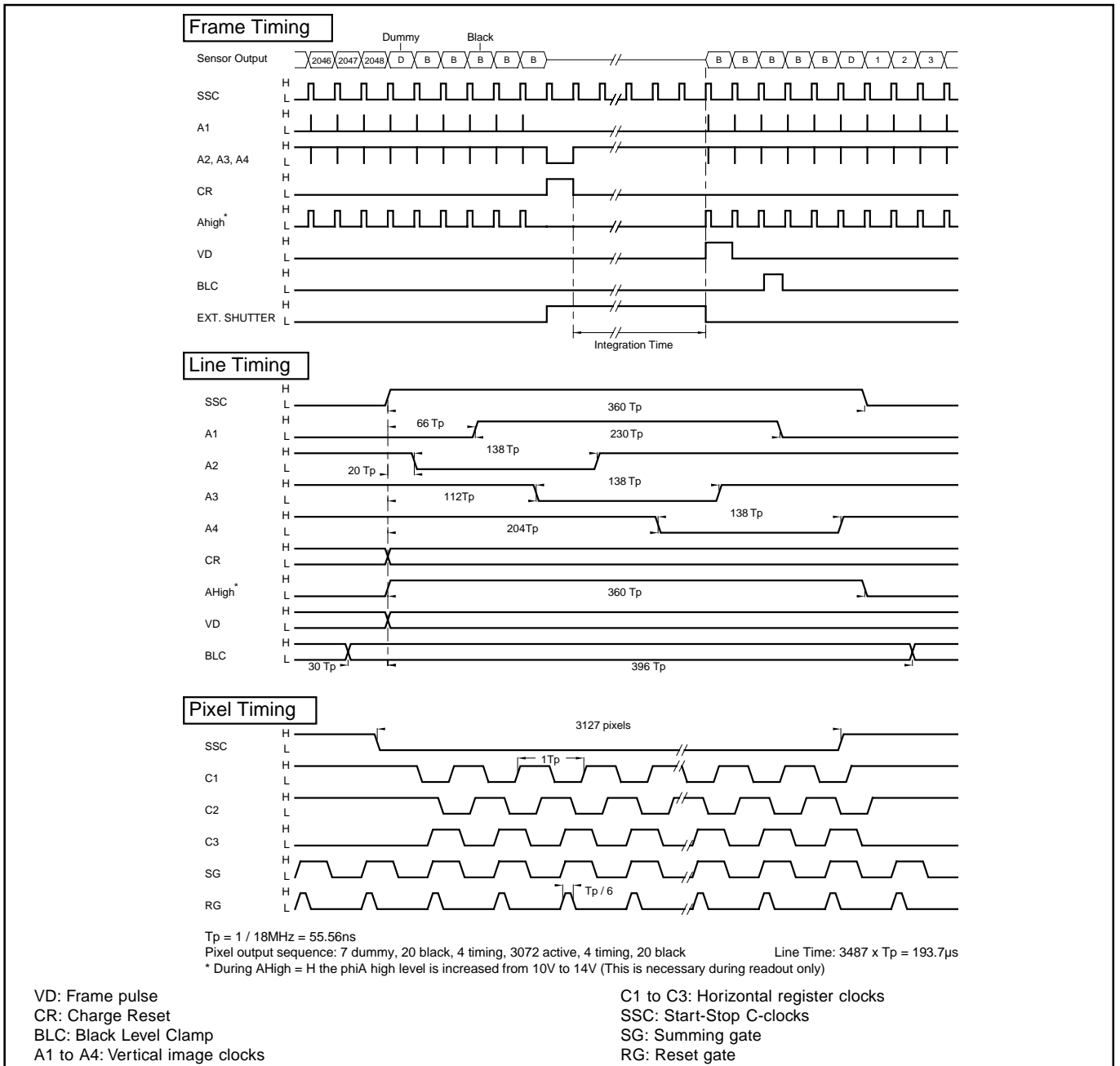
Figure 3 - Timing diagrams
